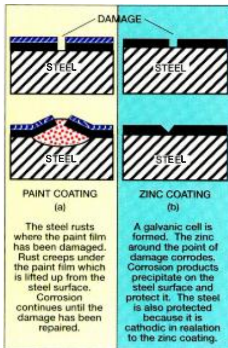
Figure 1. Cross-section showing the effect of surface damage on different rust-preventive coatings.
