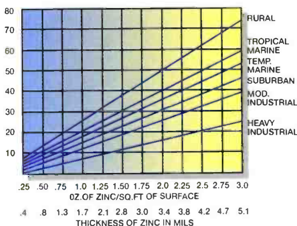
Figure 2. Service life of protective coatings vs. the zinc thickness and type of atmosphere.
